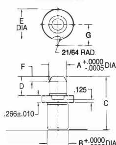
Lockscrew-Type Round Pin
