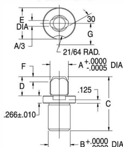
Lockscrew-Type Diamond Pin
